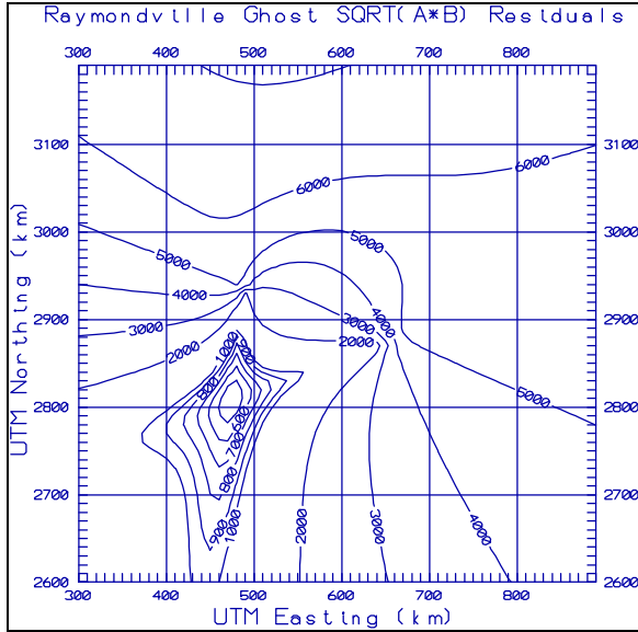
Figure 8. Correlation of Both TOA Residual Sets
