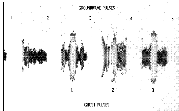
Figure 2. Raymondville Ghost: First Three Pulses
