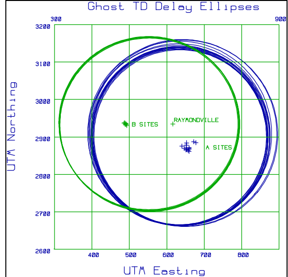
Figure 7. TD Delay Ellipses
