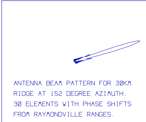
Figure 10. Antenna Beam Pattern
