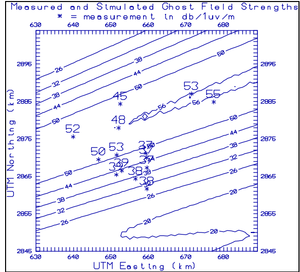
Figure 12. Brownsville Area Simulated and Measured Ghost Field Strengths
